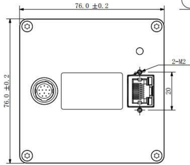
BOTTOM VIEW
